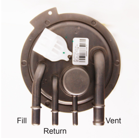
Stock sending unit configuration
